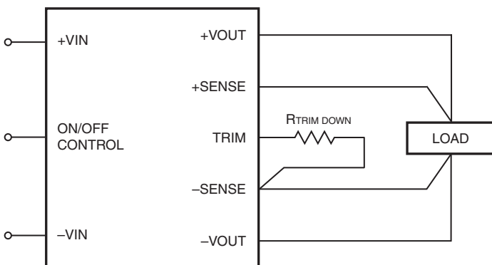
Figure 9. Trim Connections To Decrease Output Voltages
